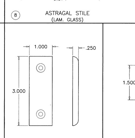
RESTRAINING PLATE
