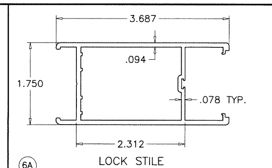
LOCK STILE (INSUL. LAM. GLASS)
