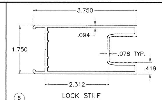
LOCK STILE (LAM. GLASS)
