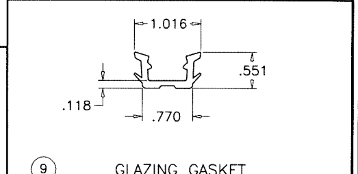
GLAZING GASKET (LAMINATED GLASS)
