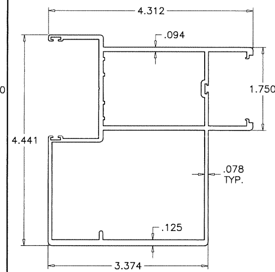
ASTRAGAL STILE (INSUL. LAM. GLASS)
