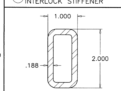
INTERLOCK REINFORCING
