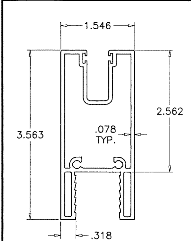
PANEL TOP RAIL (LAM. GLASS)
